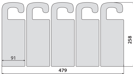
K-102-A3(5)-D-3 479*258
