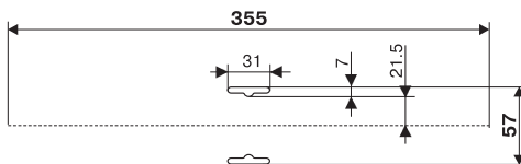
B-72-A3(5)-D-1 517*32
